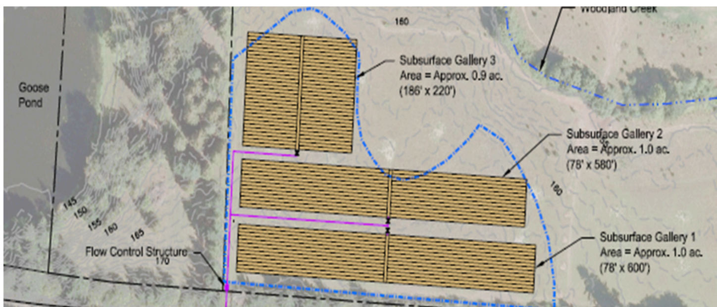
Woodland Creek Infiltration Gallery Design Layout
